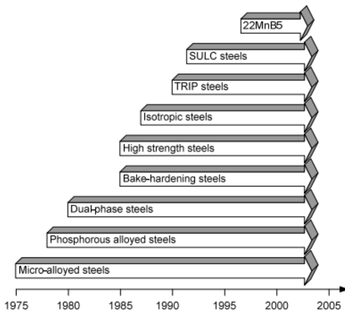
Figure 5 – Steel developments for the automotive industry during the last 30 years [7]
