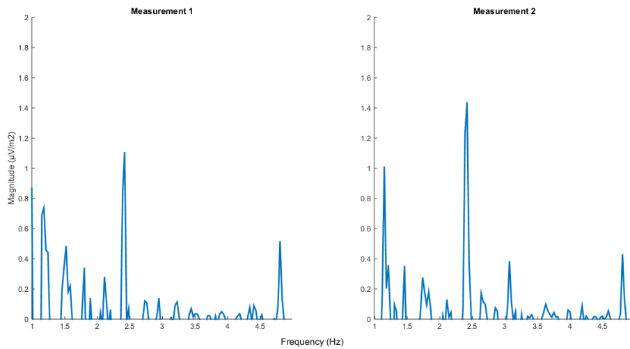
Figure 1. Group-level noise-corrected EEG frequency spectrum averaged across all channels for the two measuring sessions.
