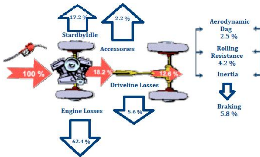
Figure 2 Overview of Energy Conversion Efficiencies in a Vehicle [5]
