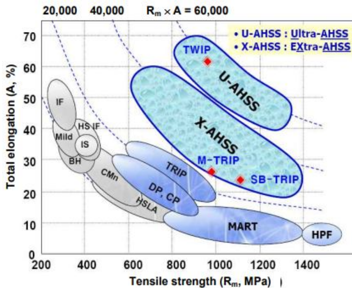
Figure 6 – Tensile strength vs. total elongation for X-AHSS and U-AHSS [7]
