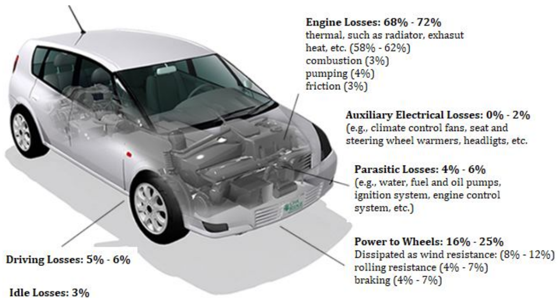
Figure 1 The energy requirements for combined city/highway driving [2]
