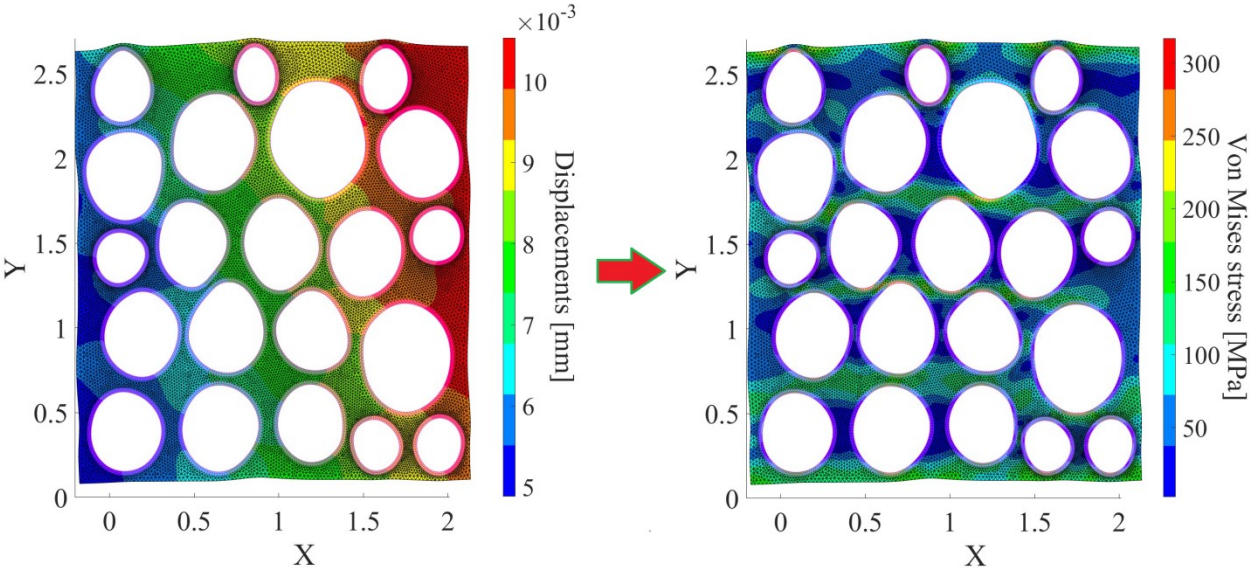
Fig. 7 Stress field converted from the displacement field of the selected SFE
