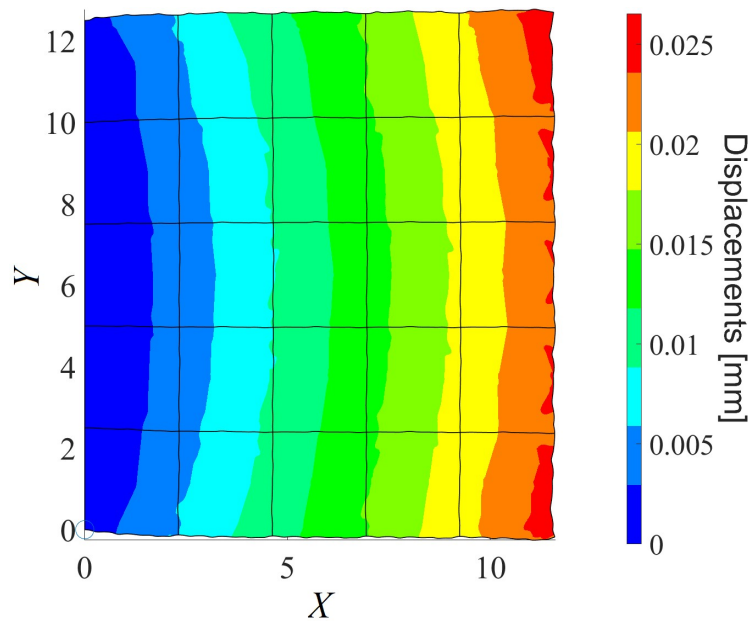
Fig. 5 Displacement field of the model built from the SFEs
