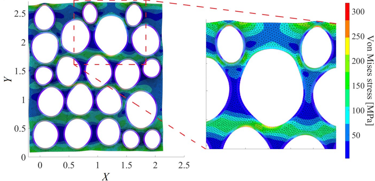
Fig. 8 The stress-reducing effect of aligned hollow spheres
