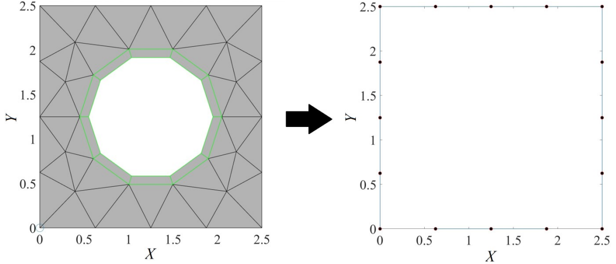
Fig. 1 Meshed substructure and its SFE
