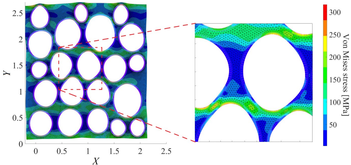
Fig. 9 Stress-increasing effect of hollow spheres at 45 degrees to the load direction
