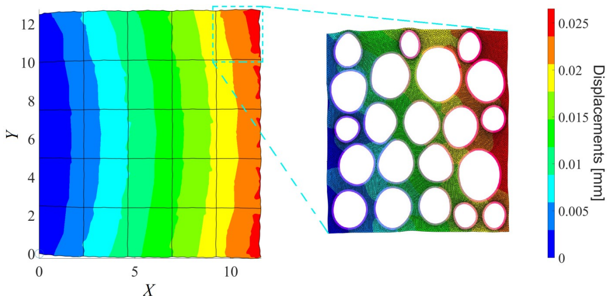
Fig. 6 The complete displacement field of a selected SFE
